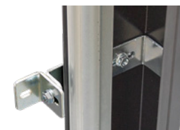
Between fix bracket shown from both sides on a no-hole frame leg.
