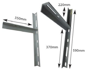
Up & down brackets
