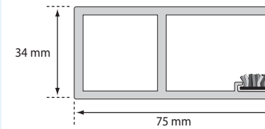
75 mm guide rails supplied as standard on SeceuroGlide Manual
