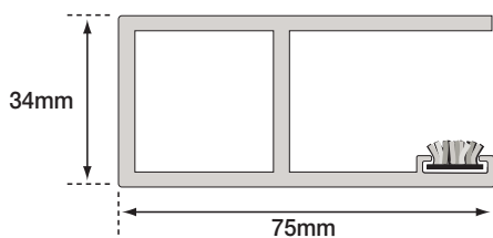
75mm guide rails supplied as standard on SeceuroGlide Manual
