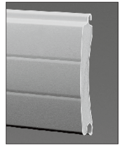
Foam filled aluminium slats typically finish 150mm above the opening to improve weather seal.
